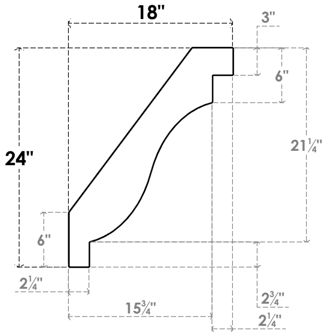
SIDE PROFILE
